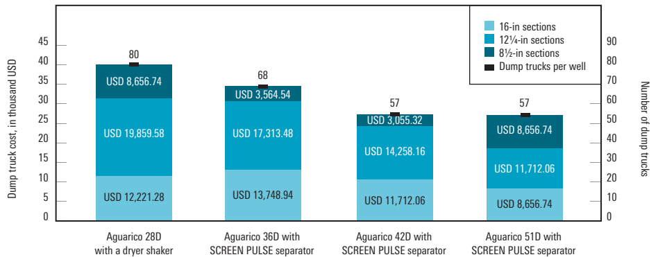
Deploying the SCREEN PULSE separator helped Conсорcio Shushufindi reduce the total mud on cuttings and cut down on the costs associated with waste disposal.
